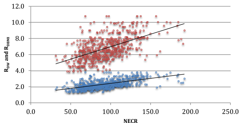
Figure 6 Graphic showing the relations between R_{DW} (blue circle) and R_{DBI} (red circles) and NECR.
